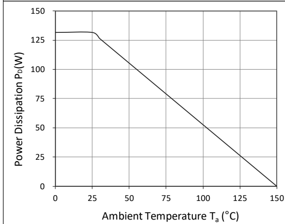
Figure 9. Power Dissipation
