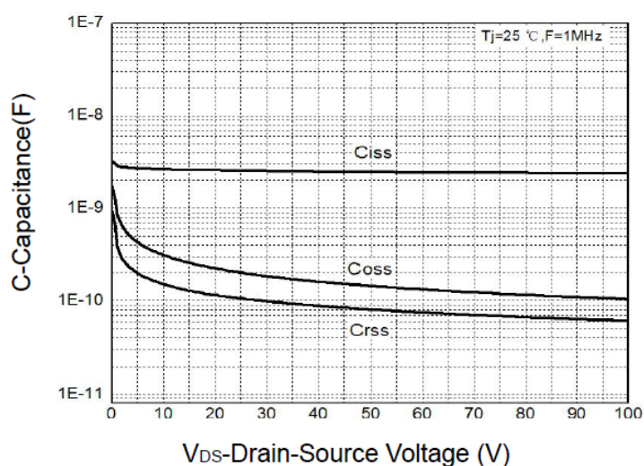
Figure 9: Capacitance Characteristics
