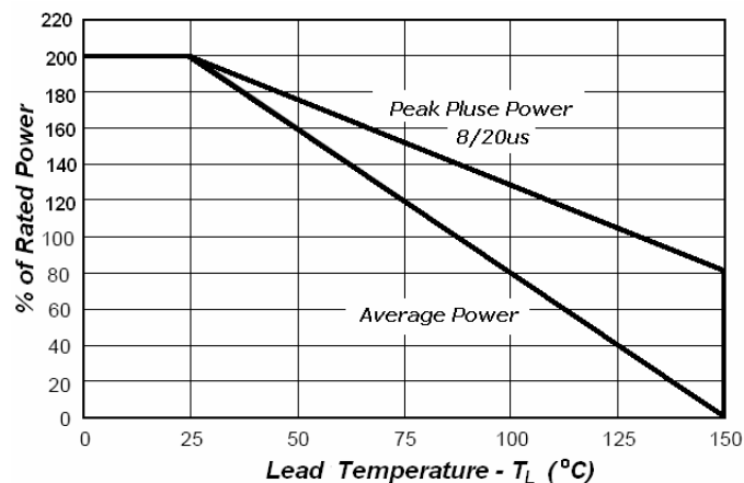
Fig2.Power Derating Curve
