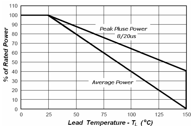
Fig3.Power Derating
